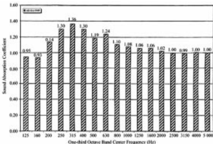
GreenSound Natural Fiber Insulation (Thickness 4") Type A Mounting, AS-SA1949; NRC 1.15
