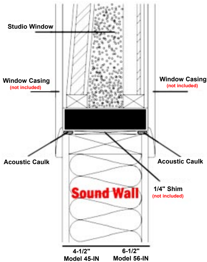
Installation Detail – Sill Type A
