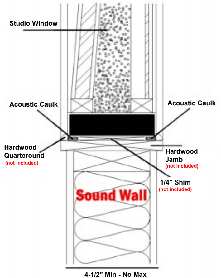
Installation Detail – Sill Type B
